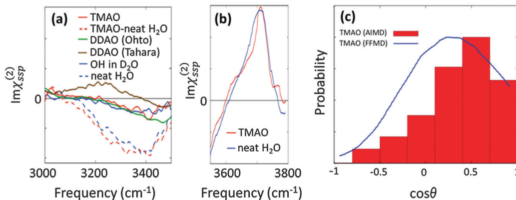
Fig. 7 (a) Experimental SFG spectra ( \text{Im}\chi_{ssp}^{(2)}(\omega) ) in the hydrogen bonded O–H stretching mode region. The TMAO solution–air interface for neat H 2 O (red broken line) and isotopic diluted water (red solid line), the water/air interface for both pure water (blue broken line) and isotopic diluted water (blue solid line), and the DDAO/isotopic diluted water interface (green and line). The DDAO spectral amplitude was normalized to the same C–H negative amplitude as TMAO. Note that the frequency range covered in the experiment is given by the finite bandwidth of the IR pulse. The data are obtained from ref. 27, 74, 78, and 79. (b) Experimentally measured \text{Im}\chi_{ssp}^{(2)}(\omega) for the free O–H stretching mode. 74 (c) Probability distribution of the angle formed by the N–O group of TMAO at the interface and the surface normal, which is denoted by red bars. 27 The angle distribution with the force field MD (3 M TMAO concentration) was taken from ref. 80 for comparison, and is shown as the blue line.
