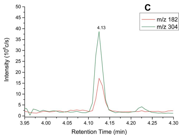
Fig. 2 Extracted ion chromatograms (XIC) for (A) cocaine and (B) benzoylecgonine in blank urine. XICs for (C) cocaine and (D) benzoylecgonine in spiked ( 200 \text{ ng ml}^{-1} cocaine and benzoylecgonine) urine standard.
