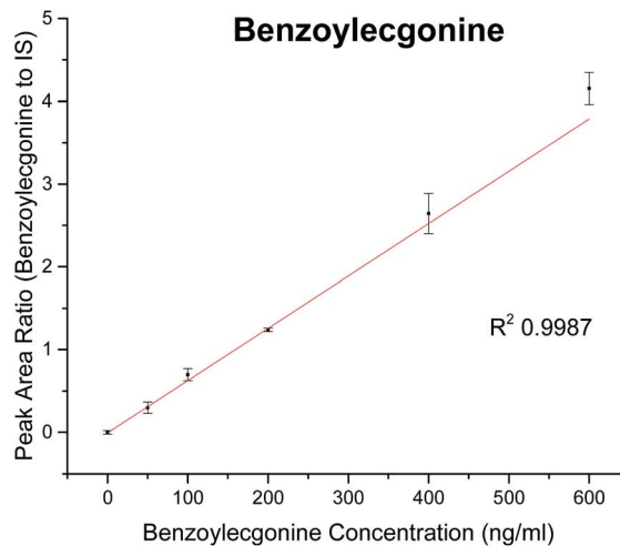
Fig. 3 Calibration curve for cocaine ( m/z 182) and benzoylecgonine ( m/z 168) in pooled urine analysed using Plate Express™ coupled with an expression compact mass spectrometer (CMS) with cocaine- d_3 ( m/z 185) internal standard.
