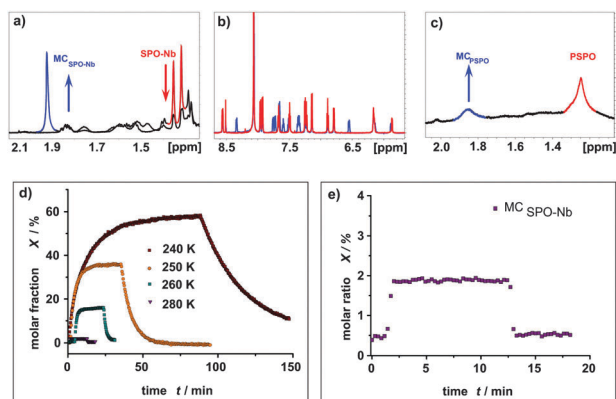
Fig. 5 (a) ^1\text{H} -NMR spectra of SPO-Nb solution in DMF- \text{d}_7 measured at 240 K prior to (red) and during irradiation (blue) with UV light ( \lambda = 365 nm). (a) Aliphatic region with a severe signal overlap of the two methyl group resonances of the SPO-Nb and resonances of the N -bound aliphatic side chain. (b) Aromatic region with well separated signals for SPO-Nb and \text{MC}_{\text{SPO-Nb}} . (c) ^1\text{H} -NMR spectrum of the PSPO polymer in DMF- \text{d}_7 at 240 K during irradiation with UV light with highlighted signals of SPO (red) and \text{MC}_{\text{SPO}} (blue). (d) Molar fractions of \text{MC}_{\text{SPO-Nb}} at different temperatures approximated from the integrals of corresponding resonances in a series of ^1\text{H} -NMR spectra. (e) Molar fraction of \text{MC}_{\text{SPO-Nb}} at 280 K.
