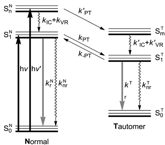
Fig. 1 A schematic representation of the energy levels describing the formation of the tautomer (T) in the S_1^T excited state caused by excitations into the S_1^N and S_2^N states of the normal (N) form. 24 k_r and k_{nr} : radiative and nonradiative (proton-transfer rate excluded) decay rates, respectively. k_{IC} : the internal conversion rate, k_{VR} : vibrational relaxation rate (solvent relaxation implicitly included in this scheme), k_{PT} and k'_{PT} : forward proton transfer rate, k_{-PT} : reverse proton transfer rate. Note that for the cases of 3-HTCA and 3-HTC-DiCN k_{-PT} is virtually zero. Please see text for detailed explanations.
