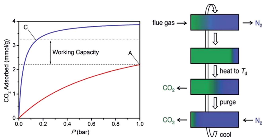
Fig. 10 (Left) CO 2 adsorption isotherms at 40 °C and 150 °C. Reprinted from ref. 59. Copyright 2012 American Chemical Society. (Right) Schematic representations of temperature swing adsorption. Reprinted from ref. 73 with permission from Royal Society of Chemistry.
