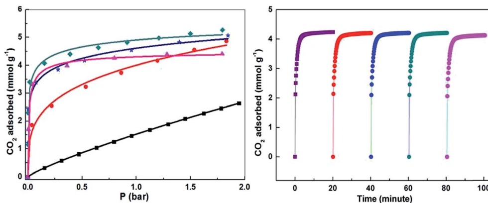
Fig. 9 (Left) CO 2 adsorption isotherms of MIL-101(Cr) before and after PEI loading at 25 °C. Symbol: ■ MIL-101, ● PEI-MIL-101-50, ★ PEI-MIL-101-75, ◆ PEI-MIL-101-100 and ▲ PEI-MIL-101-125. (Right) Cycling CO 2 adsorption kinetics of PEI-MIL-101-100. Reproduced from ref. 62 with permission of Nature Publishing Group.
