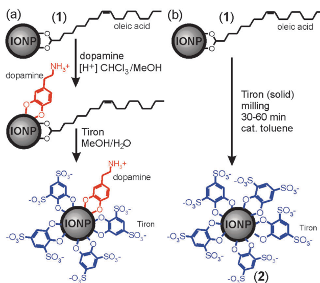
Scheme 1 Synthesis of water-soluble IONPs by: (a) two-step ligand exchange in solution, leading to exchange of oleic acid ligands 13 and (b) herein demonstrated one-step mechanochemical solvent-free process.
