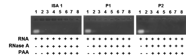
Fig. 6 Enzymatic activity of RNase A in the absence or presence of poly(amidoamine)s. Lane (1) RNA alone; (2) RNA + RNase A; Lanes (3–8) RNA + PAA: RNase A at different weight ratios: (3) 1 : 1; (4) 5 : 1; (5) 10 : 1; (6) 50 : 1; (7) 100 : 1; (8) 500 : 1.
