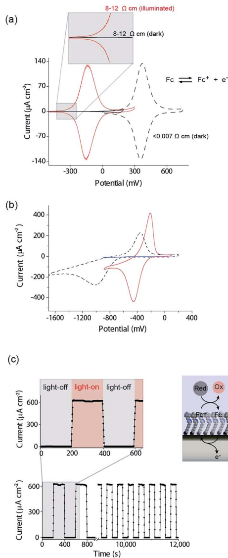
Fig. 2 (a) A cyclic voltammogram (CV) (dash black line) in aqueous 1.0 M HClO 4 at highly doped (<math><0.007 \Omega \text{ cm}</math>, dopant concentration, N_A, >8 \times 10^{18} \text{ cm}^{-3}</math>) p-Si electrodes that behave electrochemically similar to metals. A CV of a poorly doped n-Si electrode (8–12 \Omega \text{ cm} , N_D, \sim 4.5 \times 10^{14} \text{ cm}^{-3}</math>) in the dark (solid black line) and light (solid red line) at 642 nm, \sim 300 \text{ mW cm}^{-2}</math>. (b) CVs (dash black line) at highly doped p-Si electrodes (<math><0.003 \Omega \text{ cm}</math>, dopant concentration, N_A \sim 1 \times 10^{19} \text{ cm}^{-3}</math>) and poorly doped p-Si electrode (substrate: 1–10 \Omega \text{ cm} , N_A, \sim 8 \times 10^{14} \text{ cm}^{-3}</math>; illumination: 642 nm, \sim 300 \text{ mW cm}^{-2}</math>) to a surface bound anthraquinone at pH 10.1 in the dark (solid blue line) and light (solid red line). (c) Amperometric trace demonstrating the switching on and off of heterogeneous catalysis promoted by surface-bound ferrocene from an n-Si electrode to an aqueous ferrocyanide solution. The n-Si electrode is poised at +0.2 V versus Ag|AgCl| 3 M NaCl and 1 mM ferrocyanide [\text{Fe}(\text{CN})_6]^{4-} in solution recycles the ferricinium back to ferrocene with modulation of the illumination (0.1 M KNO 3 at pH 7; substrate: 8–12 \Omega \text{ cm} ; illumination: 527 nm, \sim 1.77 \text{ mW cm}^{-2}</math>, modulation is 200 s ON and 200 s OFF).
