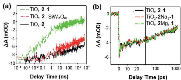
Fig. 5 (a) Ground state bleach recovery kinetics of \text{TiO}_2 - 2 (black), \text{TiO}_2 - 2-SiW}_{12}\text{O}_{40} (red) and \text{TiO}_2 - 2-1 . (b) Ground state bleach recovery kinetics of \text{TiO}_2 - 2-1 (black), \text{TiO}_2 - 2-Na}_2 - 1 (red) and \text{TiO}_2 - 2-Mg}_2 - 1 (green).
