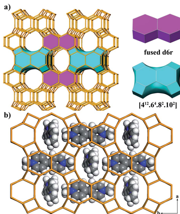
Fig. 1 (a) 3D framework of JU101 showing 10-ring channels along the [001] direction (left). Two characteristic BUs, fused d6r and the [4^{12}\cdot 6^4\cdot 8^2\cdot 10^2] cavity (right) are highlighted in the framework. (b) Simulated positions of MV^{2+} cations in the pores viewed along the [001] direction. Colour: C, gray; H, white; N, blue.
