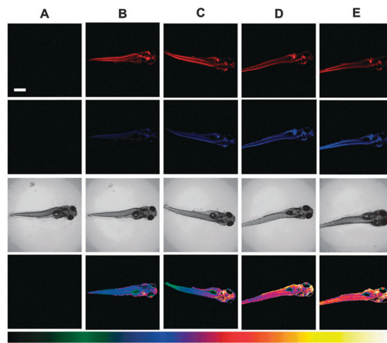
Fig. 58 Top: structure and reaction of 61 with HS − . Bottom: fluorescent images of HS − in living 5-day-old zebrafish. (A) Zebrafish only (control). The zebrafish were treated with 61 and then with various concentrations of NaSH: (B) 0 mM, (C) 10 mM, (D) 100 mM, and (E) 500 mM. First row (570–600 nm), second row (640–670 nm) and third row (corresponding DIC images). The images of the fourth row are the ratio channel. The bottom color strip represents pseudocolor correlation with HS − concentration. Scale = 500 nm. Image reproduced with permission. 230
