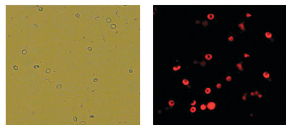
Fig. 95 Top: structure of RHO probe and related probes 90 and 91 . Bottom: (left) bright field image of PBMCs (40 \times ), (right) fluorescence image of PBMCs (40 \times ) treated with RHO . Image reproduced with permission. 320
