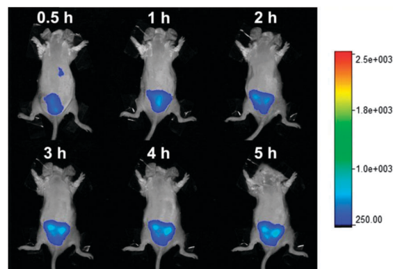
Fig. 65 Top: NIR emissive cyclen dosimeter 68 by Deng and Huang. Bottom: representative fluorescence images of mice (pseudocolour) that were injected with 68-Cu(II) (40 \mu m), followed by Na 2 S. The images were recorded after the injection of Na 2 S within 5 h. Image reproduced with permission. 238
