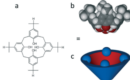
Scheme 1 (a) The molecular structure of p -iso-propylcalix[4]arene (iPc), (b) iPc shown in space filling representation and (c) iPc shown as a cone (iso-propyl groups are shown as spheres lining the upper rim).
