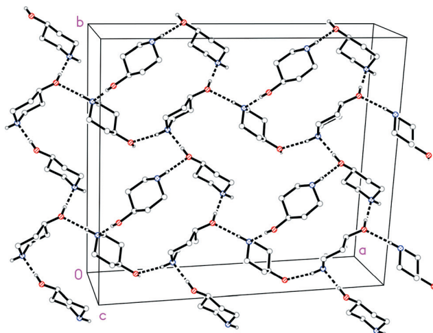
Fig. 5 Packing diagram of 1o with view direction perpendicular to the plane (\bar{1}11) . Classical hydrogen bonds are drawn as thick dashed lines. The two types of helical chain mentioned in the text run horizontally (two chains) and vertically (three chains).
