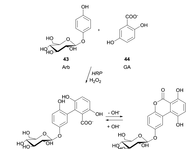
Scheme 13 Coupling of 4'-hydroxyphenyl- \beta -D-glucoside (arbutin, Arb) ( 43 ) with 2,5-dihydroxybenzoic acid sodium salt (gentisate, GA) ( 44 ).
