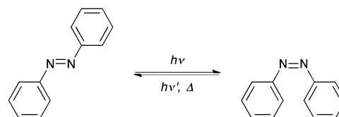
Fig. 3 Photoinduced isomerization of azobenzene.
