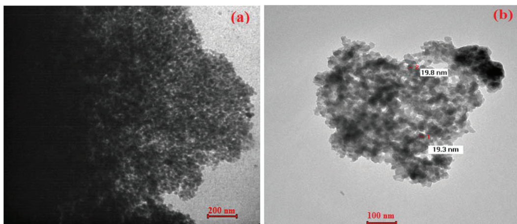
Fig. 3 TEM micrographs of (a) \text{Fe}_3\text{O}_4 -nanoparticles and (b) NP-C[8]-C 4 -COOH.
