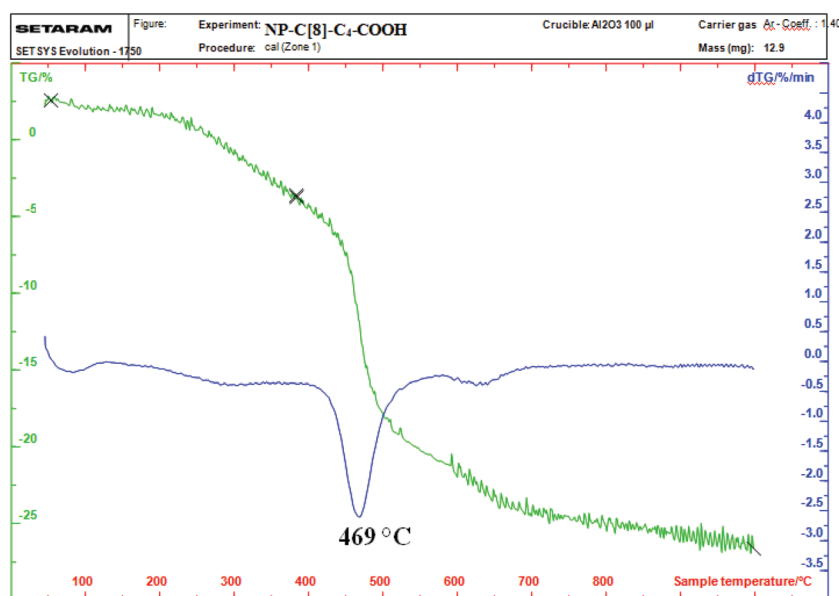
Fig. 4 TGA curves of NP-C[8]-C 4 -COOH.
