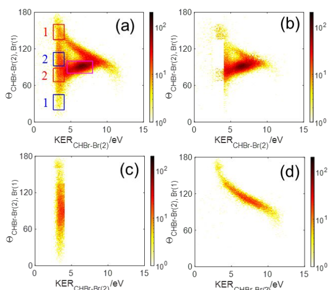
Fig. 6 Native frames analysis of the three-body fragmentation of bromoform trication into \text{Br}^+ + \text{Br}^+ + \text{CHBr}^+ assuming a \text{CHBr}_2^{2+} intermediate molecule: (a) All events, (b) after subtraction of sequential breakup via \text{Br}^+(1) + \text{CHBr-Br}^{2+}(2) and \text{Br}^+(2) + \text{CHBr-Br}^{2+}(1) , which are shown in panels (c) and (d), respectively. The red and blue rectangles shown in panel (a) mark the regions in which we replace the events within the regions marked in red by the equivalent events from the blue regions labeled with the same number to avoid contributions from other overlapping processes (see text). The magenta rectangle marks the region used to select concerted events.
