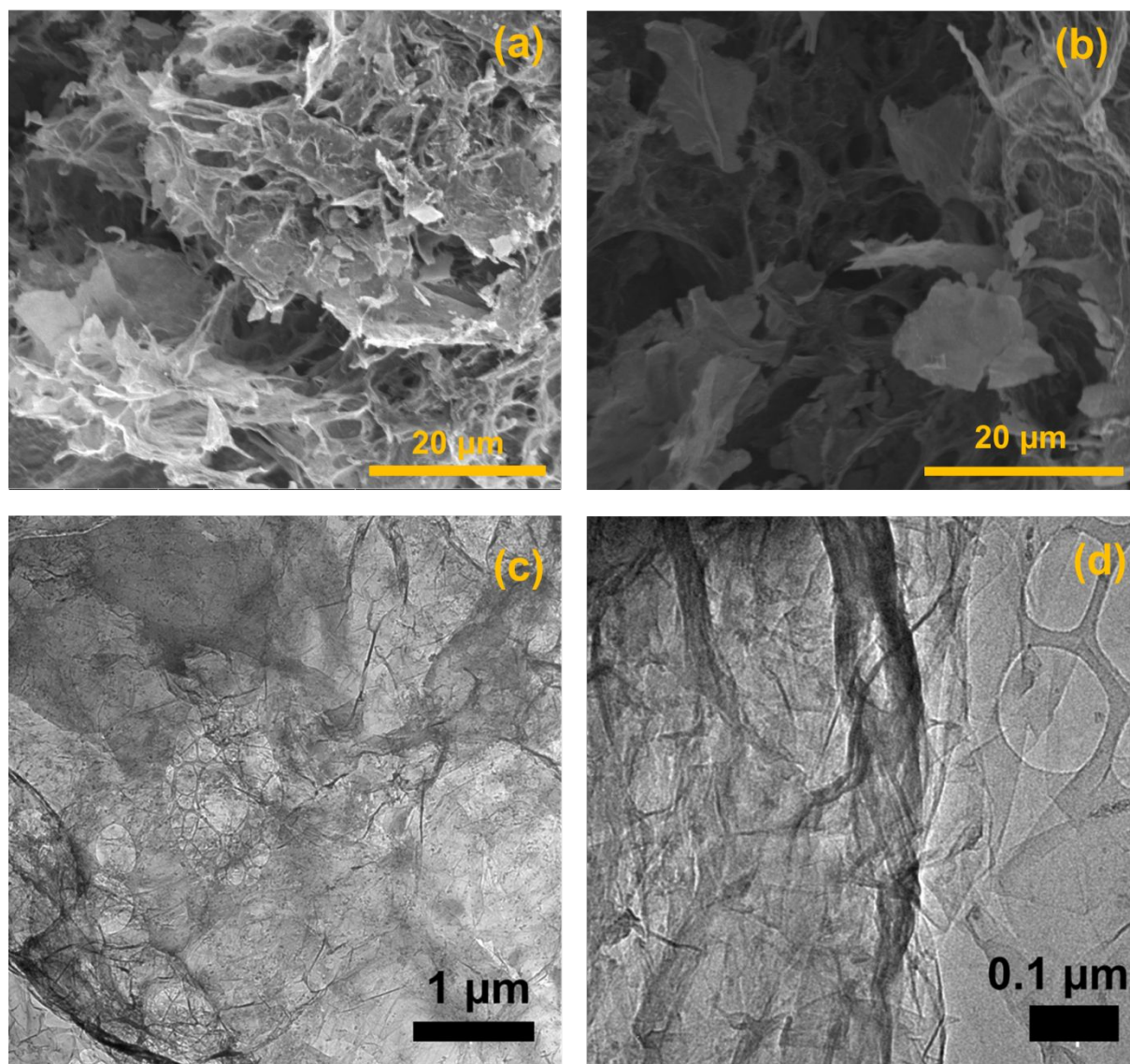
Figure 2. (a, b) FE-SEM images of GM2 gel and (c, d) TEM image of GM2 gel.
