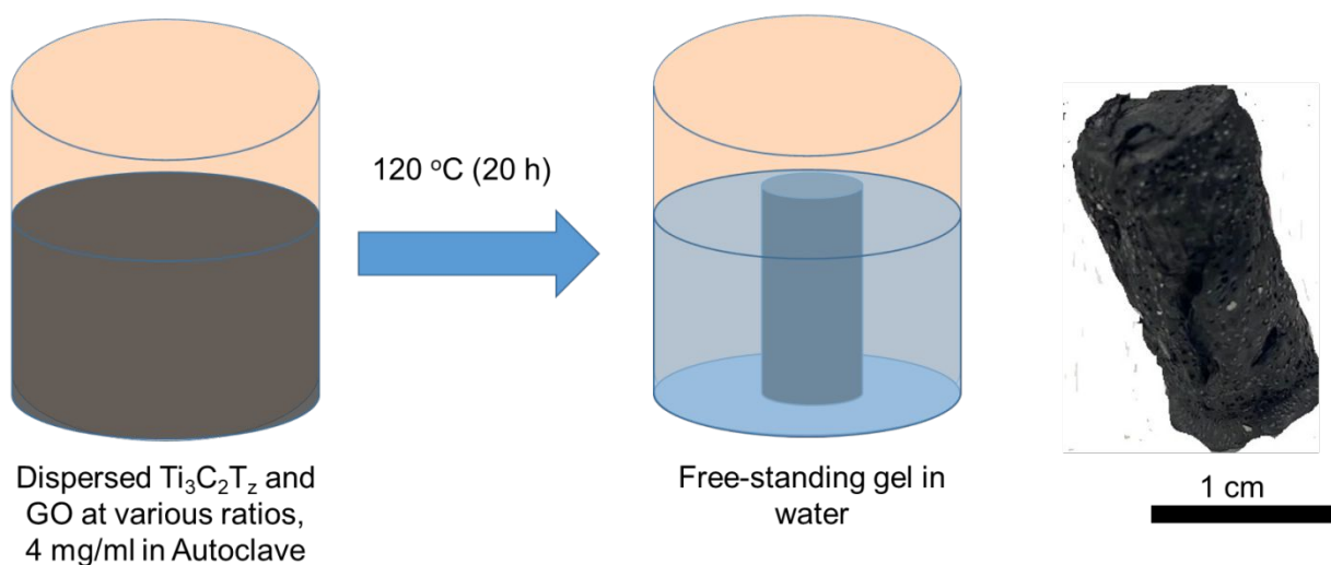
Figure 1. One-step hydrothermal synthesis process for \text{Ti}_3\text{C}_2\text{T}_z/\text{rGO} gel. The gel was collected from the autoclave and dried in a freeze-drier for 24 h.
