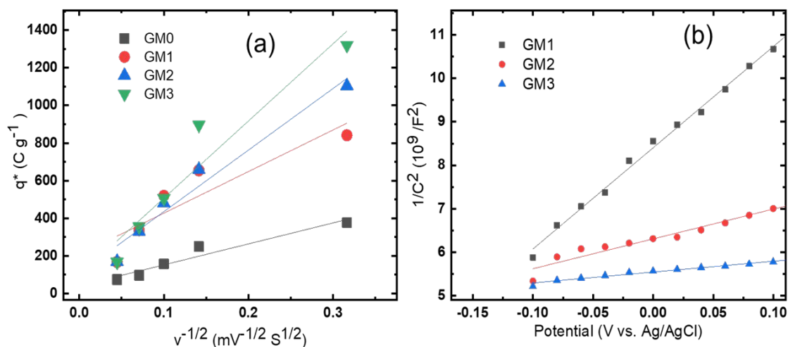
Figure 6. (a) Variation of the voltammetric charge ( q^* ) with respect to the scan rates ( v ); the lines indicate a linear fit; and (b) Mott-Schottky plot (variation of 1/C^2 vs. V ).
