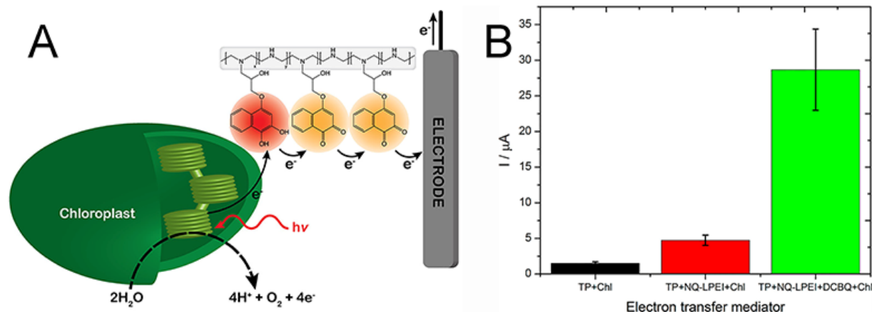
Fig. 7 A) Artificial PEET process through the naphthoquinone-based redox polymer that harvest photoexcited electrons from intact chloroplast and shuttle them to the electrode surface. B) Comparison of photocurrent generation from chloroplasts in direct electron transfer condition (TP+Chl, black), in the presence of the naphthoquinone redox polymer (TP+NQ-LPEI+Chl, red), and in the presence of both the redox polymer and diffusible dichloro benzoquinone (TP+NQ-LPEI+DCBQ+Chl, green). Adapted with permission from K. Hasan, R. D. Milton, M. Grattieri, T. Wang, M. Stephanz and Shelley D. Minter, Photobioelectrocatalysis of Intact Chloroplasts for Solar Energy Conversion. ACS Catal. , 2017, 7, 2257–2265. Copyright 2017 American Chemical Society. 98
