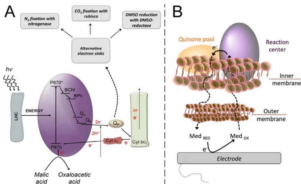
Fig. 4 A) Purple bacteria photosynthetic electron transfer chain. Light harvesting complexes (LHC); the reaction center (purple ellipse, RC) where a “special pair”, consisting of two bacteriochlorophyll molecules, absorbs light at 870 nm (P870); an excited state of the “special pair” (P870*); monomeric bacteriochlorophyll (BChl); bacteriopheophytin (BPh); a primary quinone acceptor (Q A ); a secondary quinone acceptor (Q B ); the quinone pool (Q P ); cytochrome bc1 (Cyt bc1); cytochrome c2 (Cyt c2). From the LHC, the excitation energy is transferred to the “special pair” of bacteriochlorophyll in the RC, leading to the charge separation event that is then followed by electron transfer steps, ultimately resulting in the reduction of quinone molecules in the quinone pool. A reduced quinone molecule transfers an e - and a proton to the Cyt bc1 complex that generates a proton gradient for ATP synthesis and a reduction of Cyt c2, thereby regenerating the cycle. Purple bacteria have alternative electron sinks to divert excess of electrons, through N 2 fixation, CO 2 fixation or dimethyl sulfoxide (DMSO) reduction. Adapted with permission from E. M. Gaffney, M. Grattieri, K. Beaver, J. Pham, C. McCartney and S. D. Minteer, Unveiling salinity effects on photo-bioelectrocatalysis through combination of
