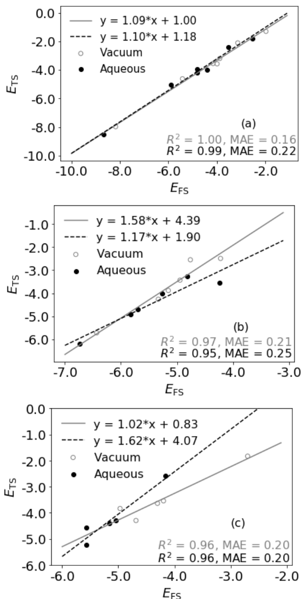
Figure 2: Regression training data (points) and linear TSS relationships (lines) for non-water-mediated dehydrogenation (a), decarbonylation (b), and hydrogenolysis steps (c) calculated under vacuum (solid lines and unfilled points) and aqueous phases (dotted lines and filled points). MAE stands for mean absolute error. Units on all values are eV.
