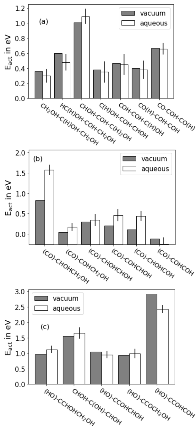
Figure 1: Comparison of activation energies calculated in vacuum (gray) and aqueous phases (white) for the non-water-mediated dehydrogenation (a), decarbonylation (b), and hydrogenolysis steps (c) calculated in this work. Bar labels are the transition states species with the species that is being removed in parentheses. Error bars denote the standard deviations of the average energies (caused by configurational fluctuations of the liquid \text{H}_2\text{O} molecules).
