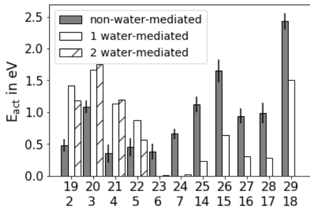
Figure 3: Comparison for activation energies for non-water-mediated (gray bars) reactions to their water-mediated (white and hashed bars) analogues. White bars indicate participation of 1 H 2 O molecule, and hashed bars indicate participation of 2 H 2 O molecules. Sets of bars are labeled by their reaction numbers. The first row of numbers are the reaction numbers for the water-mediated reactions (from Table 2), and the second row of numbers are the reaction numbers for their non-water-mediated analogues (from Table 1).
