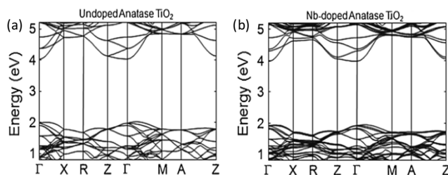
Figure 11 Calculated electronic band structures of (a) \text{TiO}_2 and (b) \text{TiO}_2:\text{Nb} . The Brillouin zone centre is denoted by \Gamma , while X, R, Z, M and A denote points at the Brillouin surface along high symmetry k-vectors in the reciprocal crystal lattice. The lines represent allowed electronic energy states at given k-points. Adapted with permission from Hitosugi et al. 89 Copyright 2008 The Japan Society of Applied Physics.
