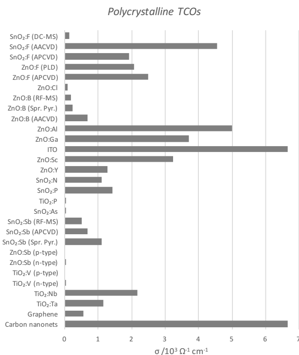
Figure 10 Comparison of conductivities of polycrystalline TCOs deposited by various means, as also compared with current carbon TCMs. The full data set with author references is given in Table 1 . Abbreviations: Aerosol-assisted or atmospheric pressure chemical vapour deposition (AA- or AP-CVD), radiofrequency or direct current magnetron sputtering (RF- or DC-MS), spray pyrolysis (Spr. Pyr.).
