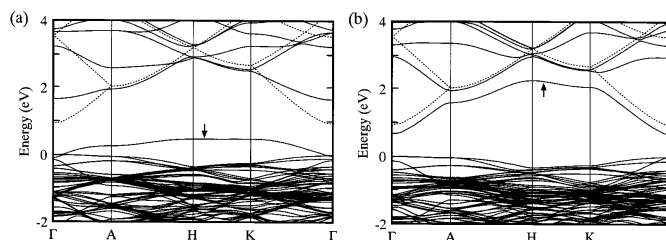
Figure 12 Calculated band structure for ZnO supercells with (a) oxygen vacancy and (b) zinc interstitial. Note the direct competition of (a) p-type and (b) n-type conductivity between the two defect species. The valence band maximum is defined as zero energy. The highest occupied state is indicated by an arrow in each. Adapted with permission from Oba et al. 99 Copyright 2001 AIP Publishing LLC.
