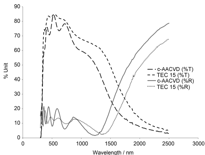
Figure 13 Optical transmittance (%T) and reflectance (%R) spectra of \text{SnO}_2\text{:F} lab-grown by combinatorial aerosol-assisted chemical vapour deposition (c-AACVD) as compared with an industrial \text{SnO}_2\text{:F} product (TEC 15, Pilkington NSG). Adapted with permission from Bhachu et al. 37 Copyright 2011 Wiley.
