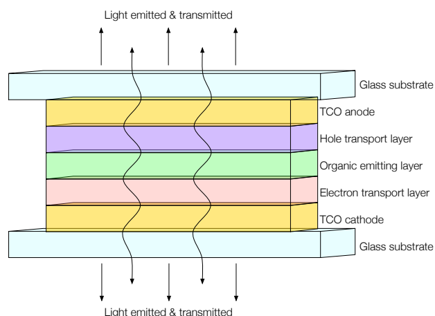
Figure 14 Schematic illustrating the construction of a transparent AMOLED device adopting TCOs for both electrodes.
