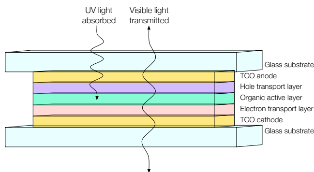
Figure 15 Schematic of a hypothetical transparent organic photovoltaic device adopting TCO materials for both electrodes.
