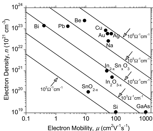
Figure 3 Boltzmann relation of electron density, mobility and hence, conductivity. The latter is displayed as straight-line contours. Adapted with permission from Edwards et al. 10 Copyright 2004 Royal Society of Chemistry.
