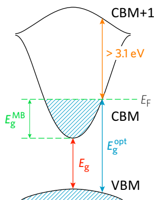
Figure 1 Diagram of the optical widening effect of the Moss-Burstein shift.
