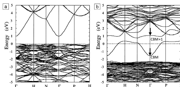
Figure 2 Band structures of (a) undoped and (b) Sn-doped \text{In}_2\text{O}_3 . The Fermi level is set at E = 0 eV. The Brillouin zone centre is denoted by \Gamma , while H , N and P denote points at the Brillouin surface along high symmetry k -vectors in the reciprocal crystal lattice. The energy lines represent allowed electronic states at given k -points. Adapted with permission from Freeman et al. 6 Copyright 2011 Cambridge University Press.
