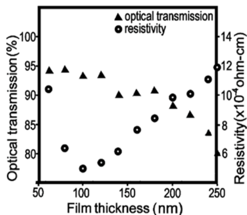
Figure 4 Effect on optical transmission and resistivity of increasing thickness of ITO film on PET substrate. Adapted with permission from Wong et al. 12 Copyright 2004 Elsevier.
