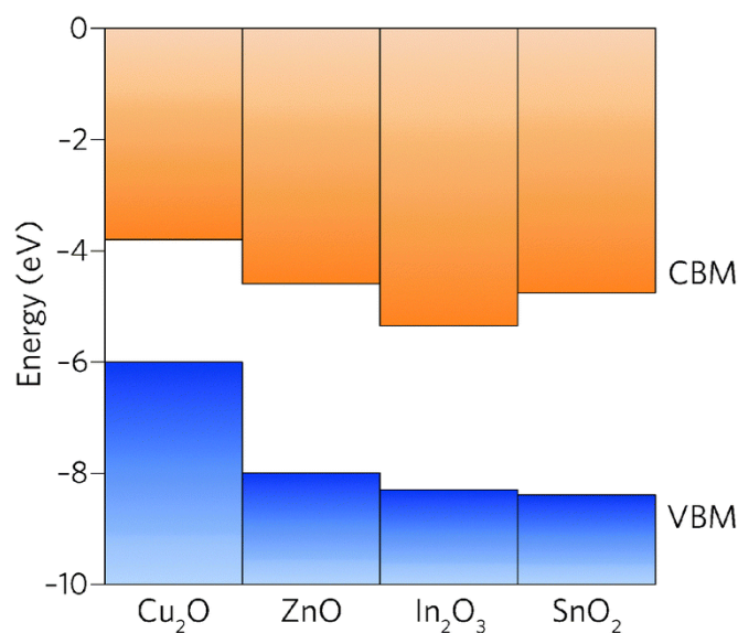
Figure 7 Calculated band gaps of common TCO host structures. The vacuum level is set at E = 0 eV. Adapted from Ganose. 2
