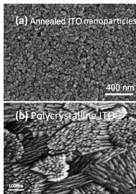
Figure 5 Scanning Electron Micrographs from (a) an ITO thin film inkjet-printed from 25 nm nanoparticles and annealed at 450°C, 28 and; (b) conventional DC magnetron sputtered polycrystalline ITO film deposited at 200°C. 27 Adapted with permission from Jeong et al. and Betz et al. 27,28 Copyright (a) 2010 and (b) 2006 Elsevier.
