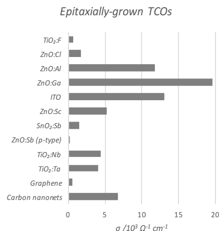
Figure 9 Comparison of conductivities of epitaxially-grown monocrystalline transparent conducting oxides, as compared with current conventional carbon-based TCMs. The full data set with author references is given in Table 1 .
