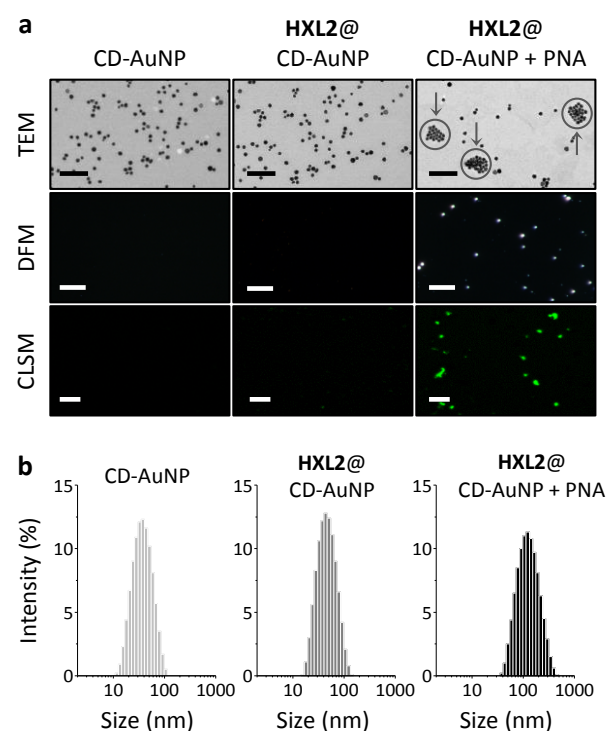
Figure 3. (a) Transmission electron microscopy (TEM, scale bar = 200 nm, arrows indicate aggregated particles), dark-field microscopy (DFM, scale bar = 20 \mu\text{m} ) and confocal laser scanning microscopy (CLSM, scale bar = 10 \mu\text{m} ) of CD-AuNP (7 nM) and HXL2@CD-AuNP (0.56 \mu\text{M}/7 nM) without or with PNA (70 \mu\text{M} ). (b) Dynamic light scattering of CD-AuNP (7 nM) and HXL2@CD-AuNP (0.56 \mu\text{M}/7 nM) without or with PNA (30 \mu\text{M} ).
