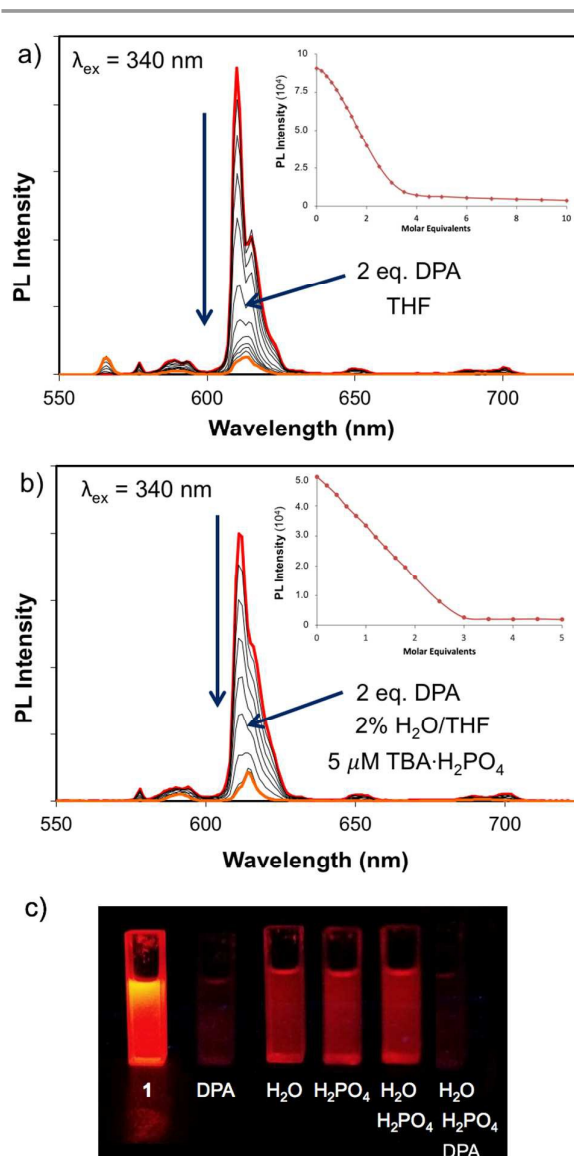
Figure 3 Fluorescence emission titration experiments where 1 (1x10 -5 M; THF) is titrated with (a) DPA (2x10 -4 M; THF) and (b) DPA (2x10 -4 M; THF) in the presence of 2% water and 0.5 equivalents of TBA-H 2 PO 4 (5x10 -6 M) at 298 K (λ ex = 340 nm). Reaction profiles are illustrated in ESI. (c) Visual comparison of emission properties of 1 upon exposure to DPA, H 2 O, and/or TBA-H 2 PO 4 .
