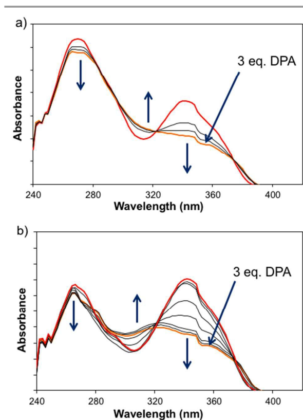
Figure 2 UV-Vis titration experiments where Eu(Tta) 3 Phen (1x10 -5 M; THF) is titrated with (a) DPA (2x10 -4 M; THF) and (b) DPA (2x10 -4 M; THF) in the presence of 2% water and 0.5 equivalents of TBA-H 2 PO 4 (2x10 -4 M) at 298 K.
