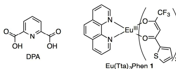
Figure 1 Chemical structures of 2,6-pyridine dicarboxylic acid (dipicolinic acid or DPA; analyte) and EuTta 3 Phen ( 1 ; sensor).
