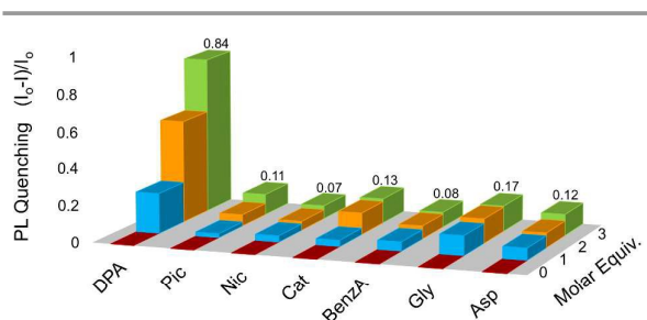
Figure 4 Selectivity study by fluorescence emission spectrophotometry assessing impact of model analytes on emission intensity of 1 ( 1 \times 10^{-5} M; THF). DPA: dipicolinic acid; Pic: 2-picolinic acid; Nic: nicotinic acid; Cat: catechol; Benza: benzoic acid; Gly: glycine; Asp: L -aspartic acid.
