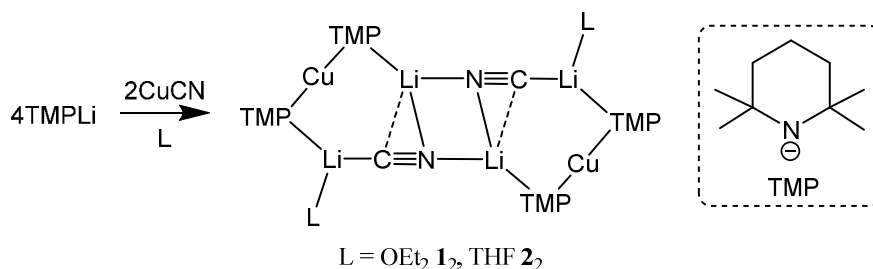
Scheme 1 Formation of the dimers of cuprates 1 and 2 .
