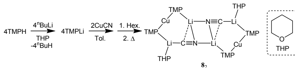
Scheme 2 Synthesis of 8 .
