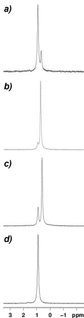
Figure 7 ^7\text{Li} NMR spectroscopic data obtained in d_6 -benzene for a) 9 , b) 10 , c) 11 , d) 12 . Sample concentrations for 9-11 were 20 mg/0.7 mL.
