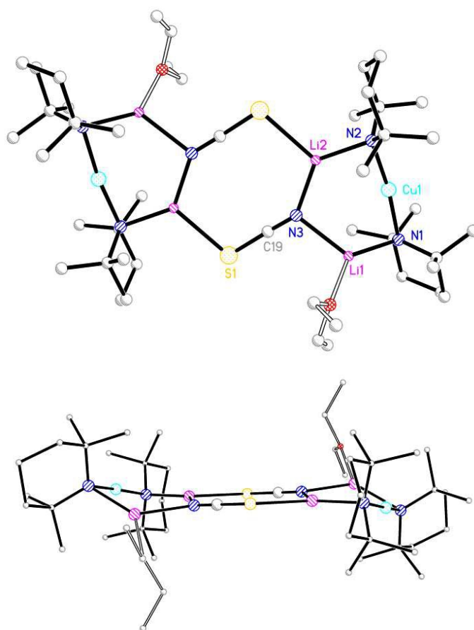
Figure 3 a) Molecular structure of \mathbf{9}_2 . H-atoms omitted. Selected bond lengths (Å) and angles (°): N1–Cu1 1.9175(18), N2–Cu1 1.9074(18), N1–Li1 2.015(4), N2–Li2 1.970(4), S1A–Li2 2.518(4), N3–Li1 2.250(5), N3–Li2 1.998(5), N3–C19 1.149(3), S1–C19 1.631(3), Cu1–N1–Li1 83.82(15), Cu1–N2–Li2 89.46(15), N1–Li1–N3 123.7(2), N2–Li2–N3 128.7(2), Li1–N3–C19 110.7(2), Li2–N3–C19 140.0(2), S1A–Li2–N3 113.17(19), Li2–S1A–C19A 103.92(13); b) side-on view emphasising the essentially flat dimer core.
