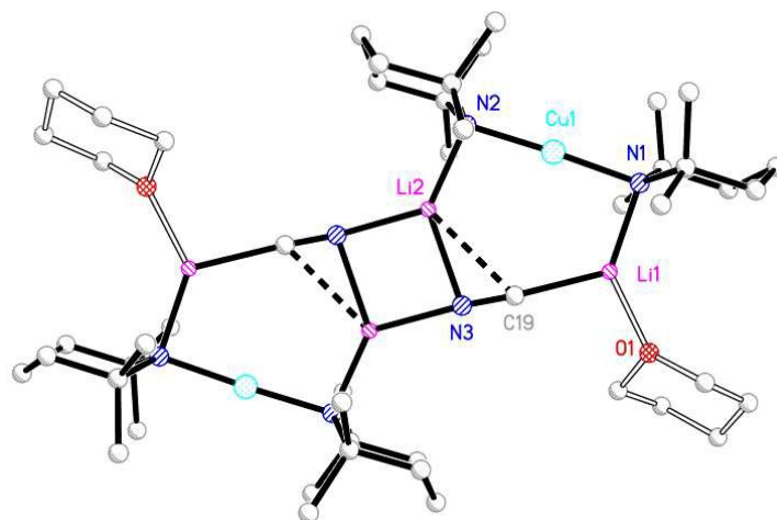
Figure 2 Molecular structure of 8 2 . H-atoms and ligand disorder omitted. Selected bond lengths (Å) and angles (°): N1–Cu1 1.950(3), N2–Cu1 1.926(3), N1–Li1 1.981(7), N2–Li2 1.951(7), C19–Li1 2.111(13), N3–Li2 2.171(13), N3–Li2A 2.047(14), Cu1–N1–Li1 90.9(2), Cu1–N2–Li2 97.2(2), N1–Li1–C19 122.3(5), N2–Li2–N3 135.2(5), N2–Li2–N3A 130.5(5).
