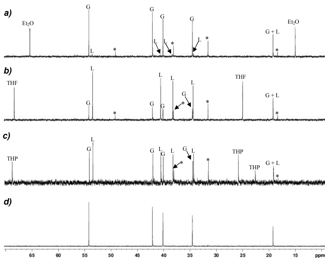
Figure 6 ^{13}\text{C} NMR spectroscopic data obtained in d_6 -benzene for a) 9 , b) 10 , c) 11 , d) 12 (*TMPH, G = Gilman, L = Lipshutz-type). Sample concentrations for 9-11 were 20 mg/0.7 mL.
