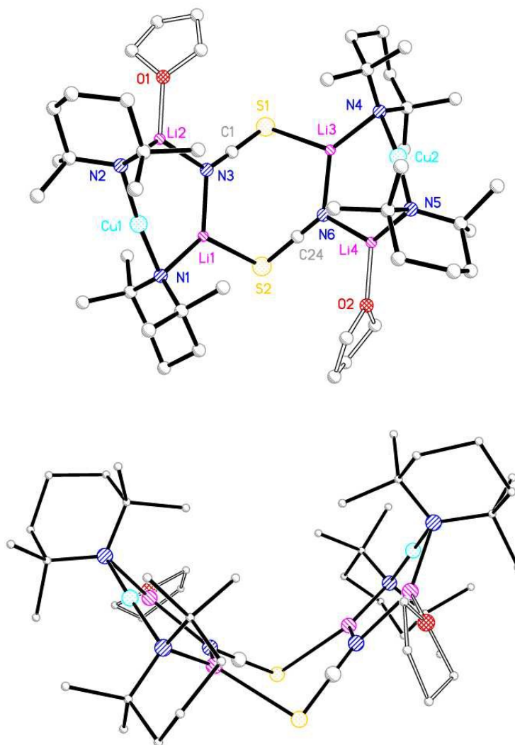
Figure 4 a) Molecular structure of 10_2 . H-atoms omitted. Selected bond lengths (Å) and angles ( ^\circ ): N1–Cu1 1.908(2), N2–Cu1 1.906(2), N1–Li1 1.977(5), N2–Li2 1.995(6), S2–Li1 2.500(6), N3–Li1 2.071(6), N3–Li2 2.105(6), N3–C1 1.159(4), S1–C1 1.627(3), Cu1–N1–Li1 87.45(18), Cu1–N2–Li2 87.66(18), N1–Li1–N3 130.7(3), N2–Li2–N3 128.9(3), Li1–N3–C1 125.0(3), Li2–N3–C1 124.8(3), S2–Li1–N3 108.8(2), Li1–S2–C24 91.72(17); b) view emphasising the boat-shaped dimer core.
