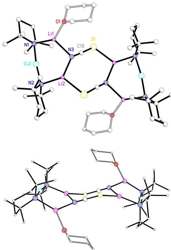
Figure 5 a) Molecular structure of 11 2 . H-atoms omitted. Selected bond lengths (Å) and angles (°): N1–Cu1 1.9204(17), N2–Cu1 1.9148(17), N1–Li1 1.990(4), N2–Li2 1.968(4), S1A–Li2 2.464(4), N3–Li1 2.164(5), N3–Li2 2.005(4), N3–C19 1.162(3), S1–C19 1.632(3), Cu1–N1–Li1 110.75(19), Cu1–N2–Li2 88.84(13), N1–Li1–N3 123.4(2), N2–Li2–N3 128.5(2), Li1–N3–C19 106.7(2), Li2–N3–C19 134.5(2), S1A–Li2–N3 107.90(18), Li2A–S1–C19 96.09(12); b) the chair-shaped dimer core.
