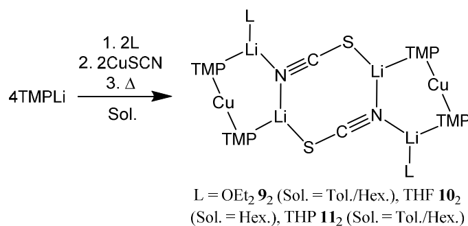
Scheme 3 Synthesis of 9-11.
