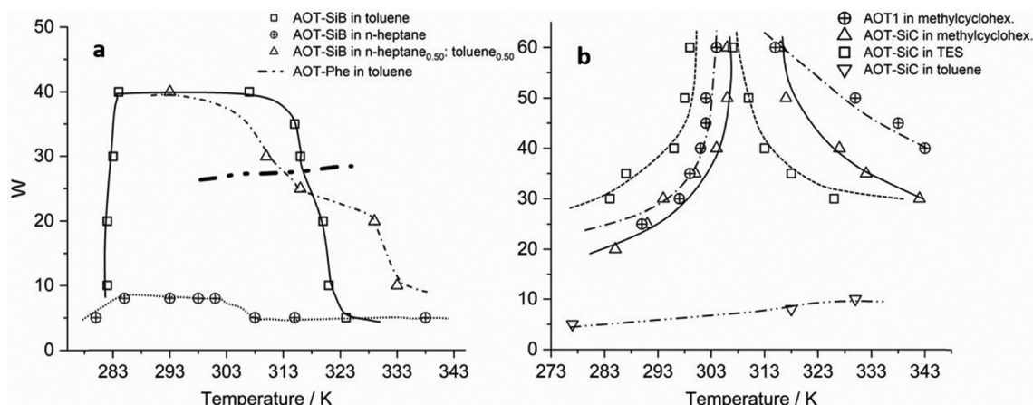
Fig. 3 Temperature–composition (T–C) phase diagrams of (a) AOT–SiB W/O-μEs in toluene, n -heptane 0.50 : toluene 0.50 [mole fraction] and pure n -heptane; AOT–Phe W/O-μEs in toluene are shown for comparison (reprinted and adapted from ref. 33 with permission, copyright 2005 American Chemical Society); (b) T–C phase diagrams of AOT–SiC-based W/O-μEs in methylcyclohexane, triethylsilane (TES, Fig. 1) and pure toluene. The phase diagram of AOT1-μEs in methylcyclohexane in (b) is shown for comparison. In (a), the area under each of the dashed curves represents a single-phase L 2 -μE. The areas outside the curves represent cloudy phases or surfactant phase separation. In (b), for each pair of the identical dashed curves for AOT–SiC μEs (and for AOT1-μEs), the T_L is represented by the boundary towards lower temperature and T_U towards higher temperature. The curves/lines are a guide to the eyes.
