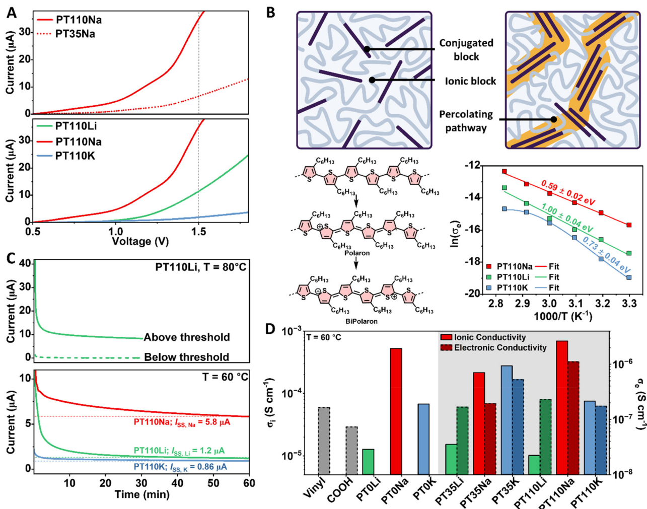
Fig. 4 Electronic conductivity. (A) Linear sweep voltammetry ( 1\text{ mV s}^{-1} scan rate) showing threshold voltages; dashed line indicates 1.5 V applied for chronoamperometry. (B) Schematic of proposed (bi)polarens and alignment mechanism, with temperature dependence of electronic conductivity and determined activation energies (eV). (C) Chronoamperometry measurements showing steady-state current ( i_{ss} ) used to determine electronic conductivity. (D) Summary of mixed conductivity at 60^\circ\text{C} including controls: vinyl-, COOH-functionalised triblock copolymers (pre-borate) and PT0 (no P3HT).
