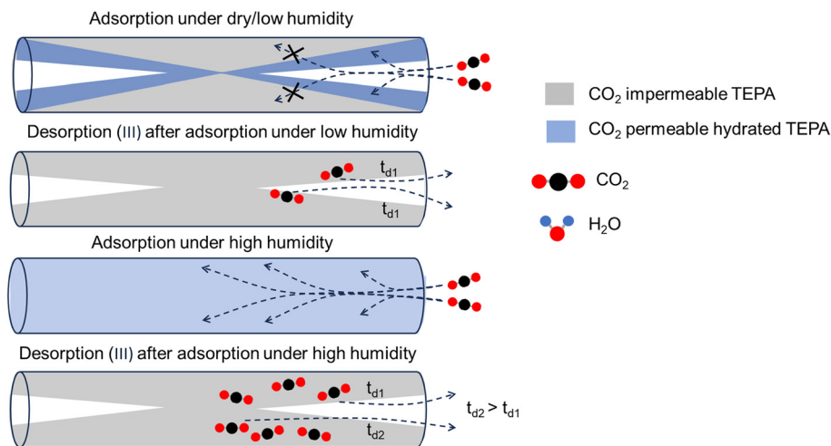
Fig. 6 Schematic illustration of CO 2 adsorption/desorption of TEPA-impregnated Mg 2 (dobpdc) under different humidities during adsorption. The annotations t d1 and t d2 represent desorption time for CO 2 desorbed from surface and buried amines, respectively. CO 2 desorption time from the surface amines should be faster than that from amines buried under surface amines.
