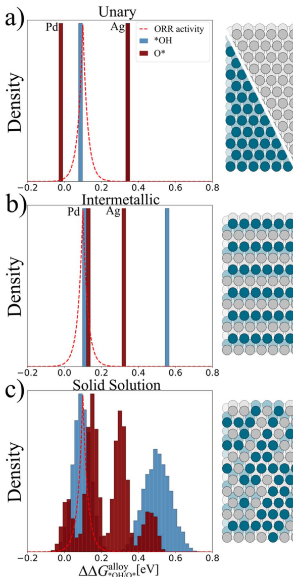
Fig. 2 Gross \ast\text{OH}/\text{O}^\ast adsorption energy distributions and illustration of the atomic configurations at the surface for (a) unary Pd(111) or Ag(111), (b) intermetallic PdAg(111), and (c) equimolar solid solution PdAg(111). In (a) and (b) it is indicated which O binding energy corresponds to which metal.
