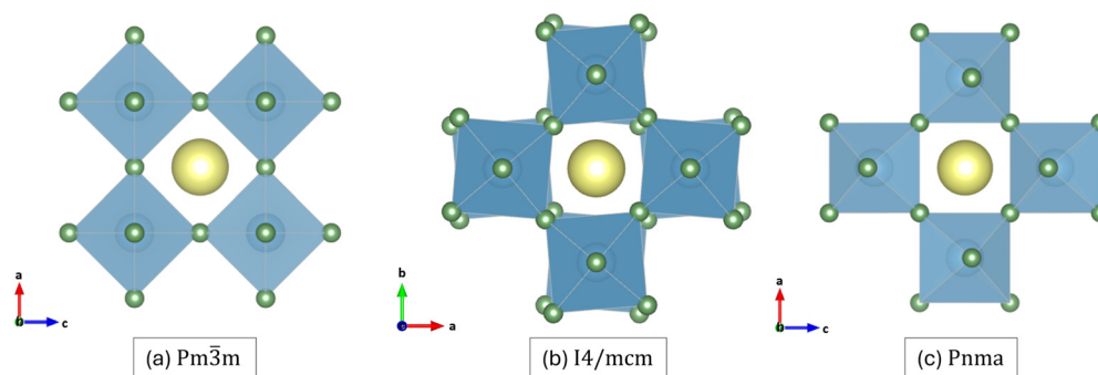
Fig. 1 Optimised structures of SrTiO 3 in the cubic Pm3m (a), tetragonal I4/mcm (b) and orthorhombic Pnma phase (c). The I4/mcm and Pnma structures are oriented to show the equivalence to the cubic structure. 71 The Sr, Ti and O atoms are shown in yellow, light blue and green respectively. These images were prepared using the VESTA software. 72
