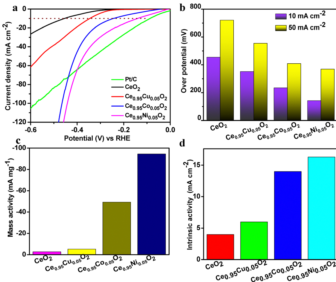
Fig. 5 (a) HER polarisation curve of the synthesized four catalysts with commercial Pt/C; (b) overpotentials; (c) intrinsic mass activity of the synthesized catalysts, and (d) intrinsic activity of the synthesized catalyst.
