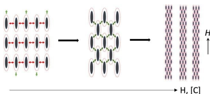
Figure 1. Schematic illustration of the formation of hierarchical tetragonal photonic crystals. Under the application of a uniform magnetic field, the \text{Fe}_3\text{O}_4@\text{SiO}_2 nanorods are magnetized with an induced magnetic dipole parallel to the external field. Driven by the dipole-dipole attractions, the nanorods assemble into tetragonal photonic crystals along a critical angle that depends on the nanorods' separation and sizes. In a strong magnetic field and a high nanorod concentration, the crystals further pack into hierarchical photonic stripes with orders across different length scales under the assistance of a template.
