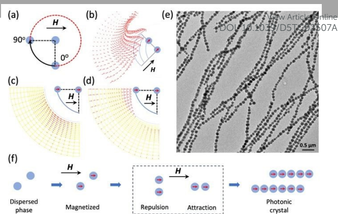
Figure 3. (a) Schematic illustration of the magnetic interactions between two nanospheres. (b) Magnetic force mapping between the two nanospheres at different angles and separations. (c) The tangent and (d) normal components of the magnetic interactions at different angles. (e) The TEM image of the assembled one-dimensional chains under a magnetic field. (f) Schematic illustration of the magnetic interactions between nanospheres and the assembly into one-dimensional photonic crystals through the end-on attachment. The nanospheres are represented by blue dots. The external magnetic field and nanospheres' induced magnetic fields are indicated by black and red arrows, respectively.
