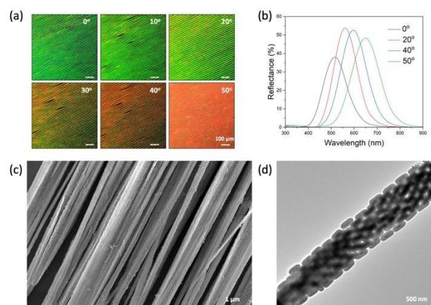
Figure 5. Assembly of nanorods into hierarchical photonic structures in a strong magnetic field under the assistance of a template. (a) Optical microscopic images of the photonic structures under different field directions. (b) The reflection spectra of the photonic structures. (c) SEM and (d) TEM image of the photonic structures in a strong magnetic field.
