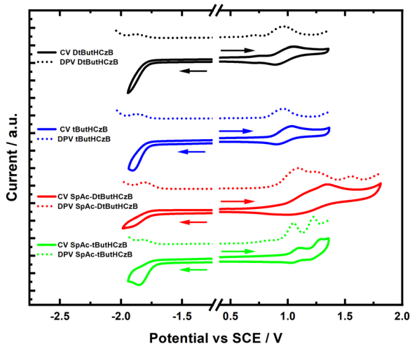
Fig. 6 Cyclic voltammetry (CV) and differential pulse voltammetry (DPV) measurements performed in DCM solution (0.1 M [ ^t\text{Bu}_4\text{N} ]PF _6 ) at a scan rate of 0.1 V s ^{-1} and referenced to SCE ( E_{\text{ox/red}} [V vs. SCE] = E_{\text{ox/red}} [V vs. Fc/Fc ^+ ] + 0.46). 39
