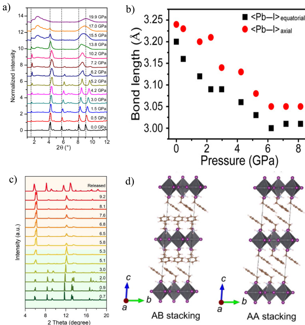
Fig. 5 Subtle structural transition of RP-type (PEA) 2 PbI 4 . (a) XRD spectra upon compression to 19.9 GPa and (b) Pb–I bond lengths as functions of pressure. Reproduced from ref. 19 with permission from American Association for the Advancement of Science, copyright 2019. (c) XRD spectra upon compression to 9.2 GPa and (d) crystal structures showing both AB and AA stacking arrangements. Reproduced from ref. 51 with permission from American Chemical Society, copyright 2019.
