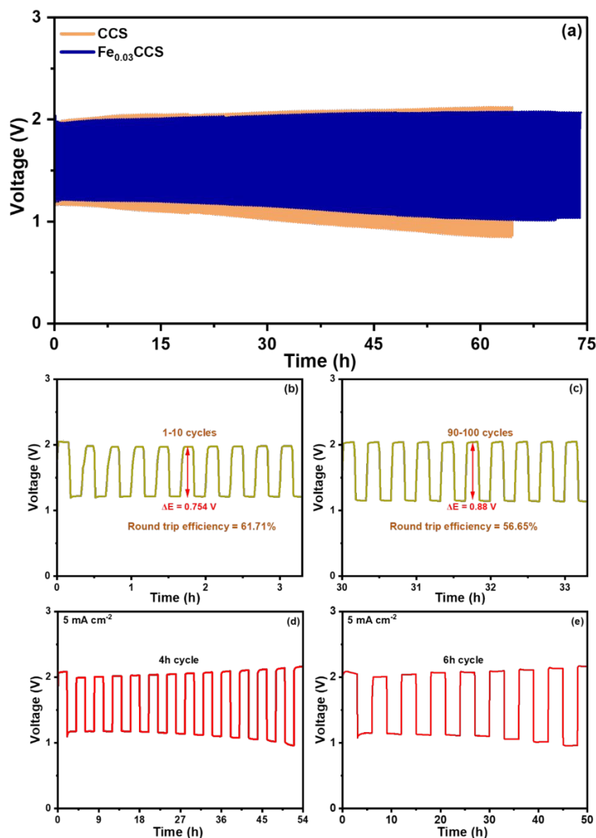
Figure 9: Galvanostatic charge discharge curve at 5 mA cm -2 for 10 minute charge discharge cycle. (b) and (c) Corresponding round trip efficiency calculation at 1-10 cycles and 90-100 cycles respectively. Galvanostatic charge-discharge plot of Fe 0.03 CCS zinc-air battery at a current density of 5 mA cm -2 with (d) 4 h per cycle (e) 6 h per cycle.
