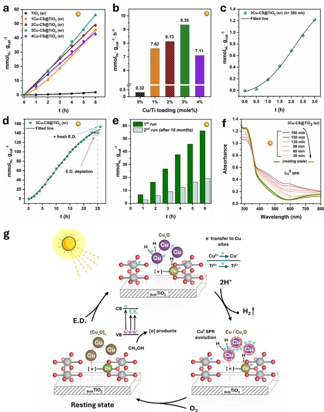
Fig. 6 (a) Performance of each synthesized photocatalyst for the photocatalytic HER under full solar light spectrum illumination over the course of 6 hours, (b) average \text{H}_2 evolution rate per hour for each photocatalyst, (c) photocatalytic HER with 3Cu-CS@TiO 2 (sr) under pure visible light (AM 1.5G filter + 380 nm cutoff), (d) photocatalytic HER with 3Cu-CS@TiO 2 (sr) over the course of 26 h solar light illumination for the determination of the rate limiting component, and (e) stability evaluation of the catalytic dispersion after 18 months. (f) Solid-state photochemical UV-DRS analysis of 3Cu-CS@TiO 2 (sr) and (g) schematic illustration of the transformations occurring on the photocatalytic surface of 3Cu-CS@TiO 2 (sr) during the solar-light driven HER.
