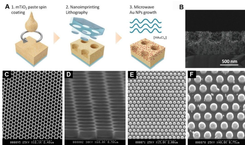
Fig. 6 (A) Fabrication scheme and (B) SEM cross-sectional image of the nanostructured photocatalytic TiO 2 photonic crystal substrates formed by using lithography approach. Reproduced with permission from ref. 50. Copyright 2021 Wiley. SEM images of (C, D) silicon on insulator photonic crystal with 500 nm lattice constant and (E, F) silicon nanoimprint mold fabricated by electron beam lithography. Reproduced with permission from ref. 94. Copyright 2004 Elsevier.
