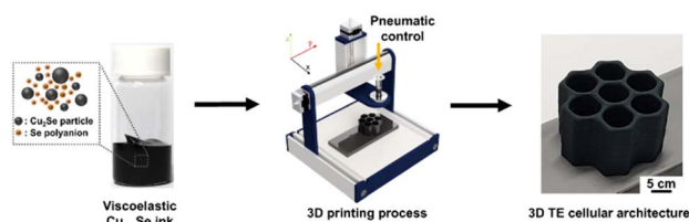
Fig. 5 Scheme for 3D printing process of the \text{Cu}_2\text{Se} -based honeycomb cellular architecture by using all-inorganic \text{Cu}_{2-x}\text{Se} ink. Reproduced with permission. 124 Copyright 2021, Springer Nature.
