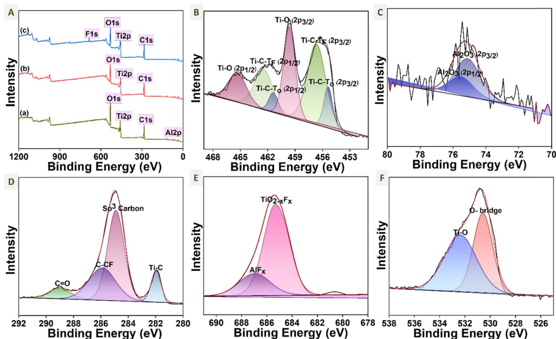
Fig. 4 Elemental composition of MSTC-0X: (A) XPS wide energy spectra of \text{Ti}_3\text{AlC}_2 , MSTC-00 and MSTC-0X (down to up). High resolution elemental (B) Ti 2p, (C) Al 2p, (D) C 1s, (E) F 1s, and (F) O 1s spectra of MSTC-0X.
