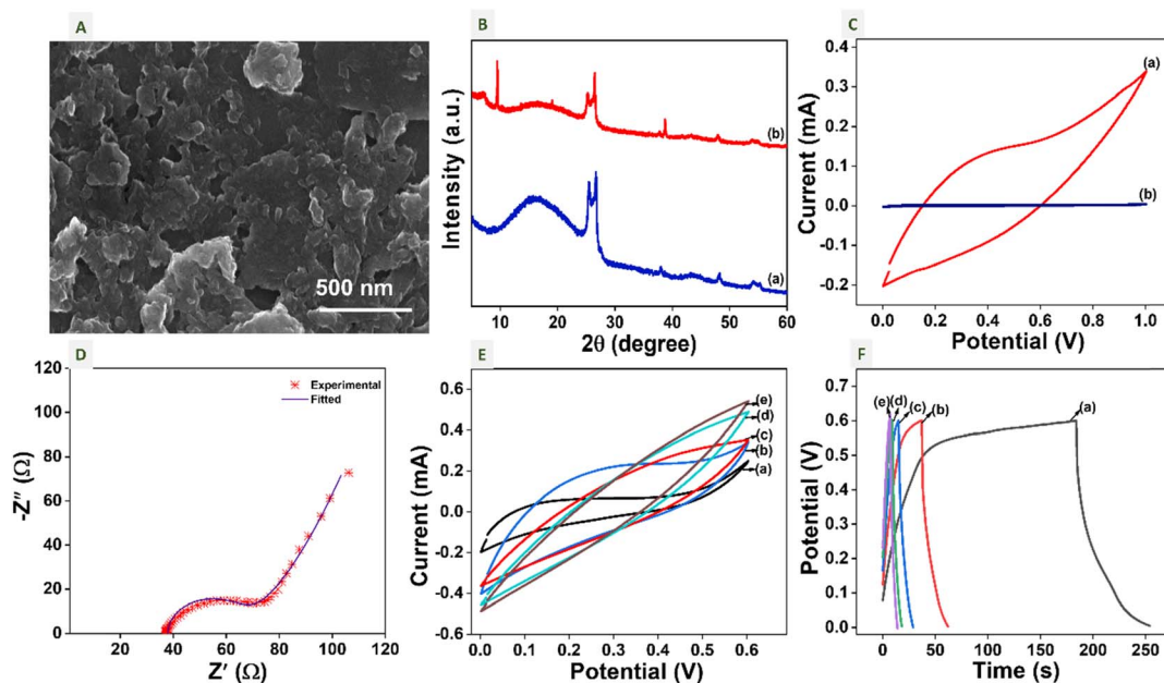
Fig. 5 Electrochemical studies of the TC-3DE electrode: (A) SEM image of EXTC-0X, (B) XRD patterns of (a) activated 3DE and (b) TC-3DE, (C) cyclic voltammograms of (a) bare activated 3DE and (b) TC-3DE, (D) Nyquist plot, (E) cyclic voltammograms at different scan rates ((a) 2, (b) 10, (c) 30, (d) 70, and (e) 100 \text{ mV s}^{-1} ) and (F) GCD curves at different current densities ((a) 200, (b) 300, (c) 400, (d) 500, and (e) 600 \text{ mV s}^{-1} ) of TC-3DE in 1 M \text{H}_2\text{SO}_4 against Ag/AgCl (3 M KCl).
