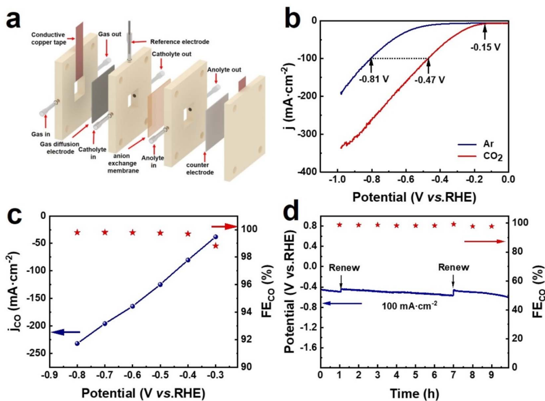
Fig. 4 (a) Schematic illustration of the flow cell electrolyzer. (b) LSV curves of the Ni-NMCF-10 catalyst under Ar or CO 2 . (c) \text{FE}_{\text{CO}} and j_{\text{CO}} with different applied potentials and (d) long-term stability tests of the Ni-NMCF-10 catalyst at 100 mA cm -2 in the flow cell.
