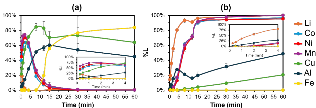
Fig. 3 Effect of varying the leaching duration on the leaching efficiencies of the (a) organic phase and (b) aqueous phase at 80 °C. Experiments were conducted using a solid-to-liquid ratio of 10 mg/mL, DES-to-aqueous phase volume ratio of 1:1, and 5 M \text{H}_2\text{O}_2 as the aqueous phase.
