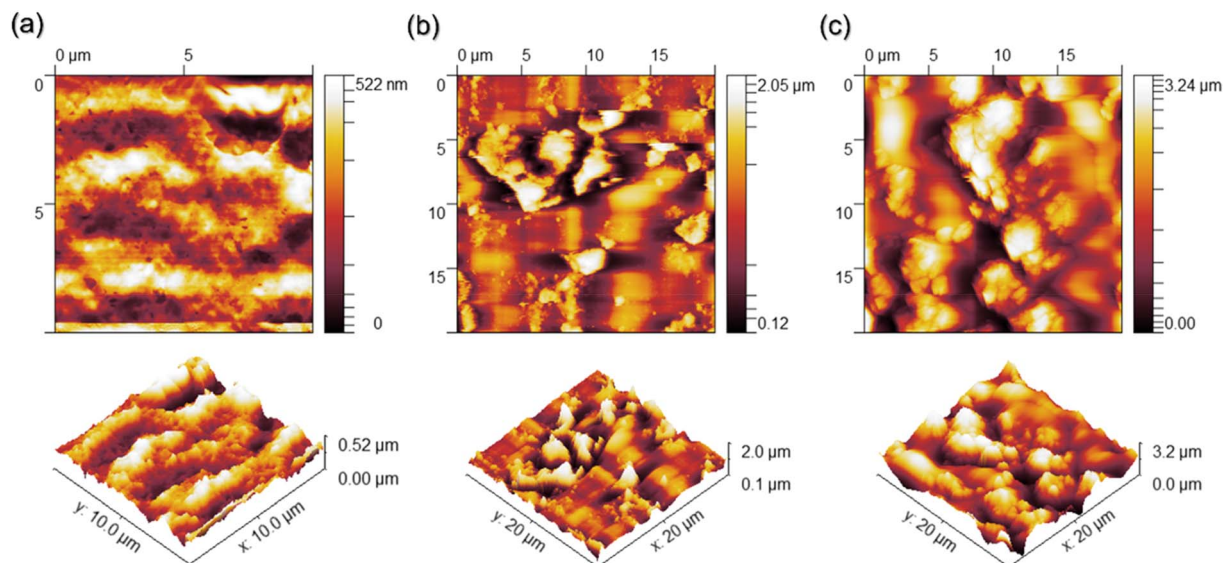
Fig. 7 AFM images of KNPs at different functionalization stages: (a) KNPs, (b) \text{Fe}_3\text{O}_4\text{@KNPs} , and (c) \text{Fe}_3\text{O}_4\text{@KNPs-Cu(II)} .
