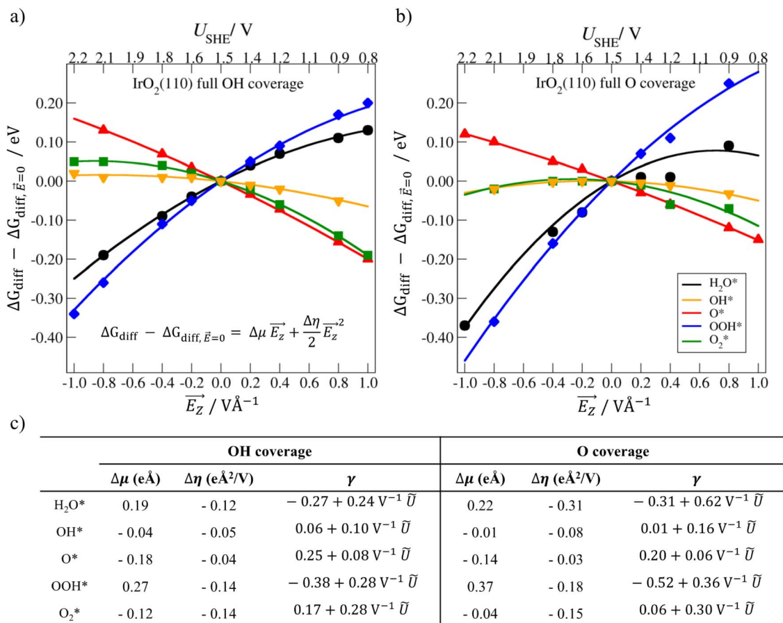
Fig. 3 Field response of the relevant intermediates in OER on \text{IrO}_2(110) under (a) \text{OH}^* coverage and (b) \text{O}^* coverage on \text{Ir}_{\text{CUS}} sites. (c) Table with fitted values for the change in surface dipole ( \Delta\mu , [eÅ]) and polarizability ( \Delta\eta , [ \frac{\text{e}\text{\AA}^2}{\text{V}} ]) associated with a change in surface phase. Additionally, the net potential response for each adsorbate is indicated where \tilde{U} = U_{\text{SHE}} - U_{\text{PZC}} .
