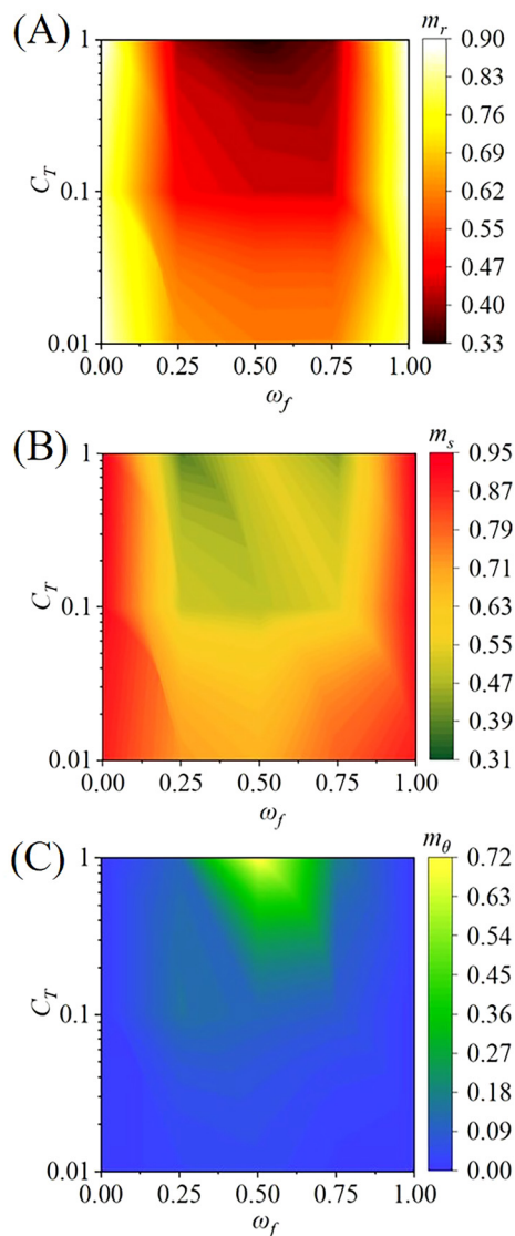
Fig. 2 The contour plots showing the variation of (A) m_r , (B) m_s , and (C) m_\theta for the dried deposit patterns formed by drying binary dispersion drops containing \text{PS}^+-\text{PS}^- ( \approx 200 nm diameter) as a function of concentration ( C_T ) and mixing fraction ( \omega_f ).
