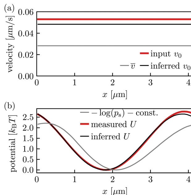
Fig. 5 (a) Inferred v_0 from driven experimental data compared to the desired input value v_0 . Though there are some statistical deviations in the values for v_0 (related to Fig. 4(b)), both obtained values for v_0 are well distinguishable from the mean velocity \bar{v} (grey line). (b) The potential U(x) inferred from the driven data via eqn (17) (black line) matches the potential measured from the equilibrium data projected on one period [0, L] using U(x) = -\ln(p_{eq}(x)) - \text{const.} (red line) quite well. The barrier height (difference between minimum and maximum) is 2.76k_B T in the red line and 2.65k_B T in the black line, respectively. It deviates from -\log(p_s) (grey line) since the driven data set does not obey a Boltzmann density [see eqn (2) and (3)].
