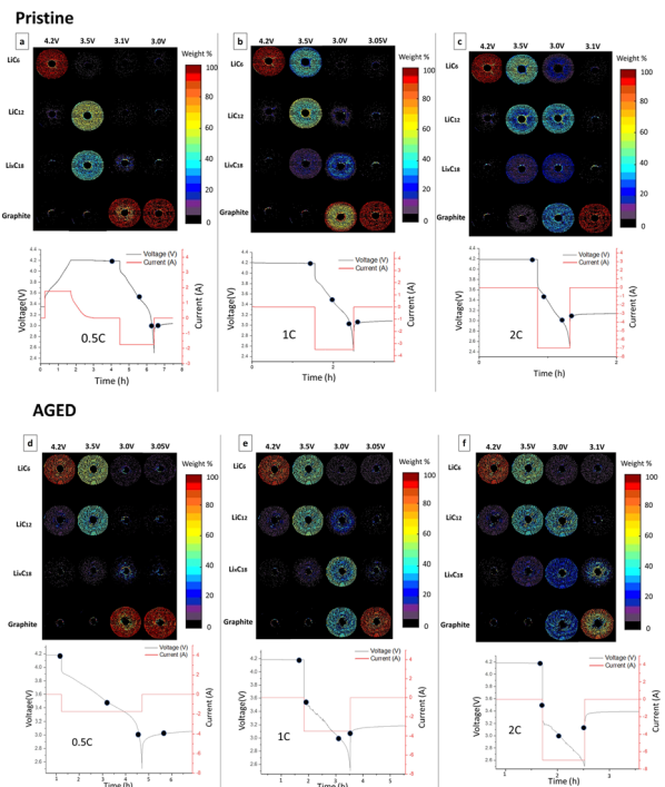
Fig. 6 Weight% distribution of different graphite phases during discharge at increasing C rates inside the pristine cell. Pristine cell is showed in (a)–(c), starting from a C rate of 0.5 to 2C. Aged cell is showed in (d)–(f), starting from a C rate of 0.5 to 2C.
