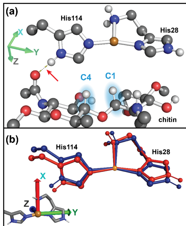
Fig. 11 (a) Optimized structure for Cu(I) SmAA10A ·chitin indicating the hydrogen-bonding interaction (red arrow) between N^{61}_{\text{His114}} and an acetamidyl O from chitin. (b) Overlay of Cu(I)- SmAA10A (blue) and Cu(I)- SmAA10A ·chitin (red) depicting the change induced in His114 upon chitin binding. The Cu site is depicted in orange.
