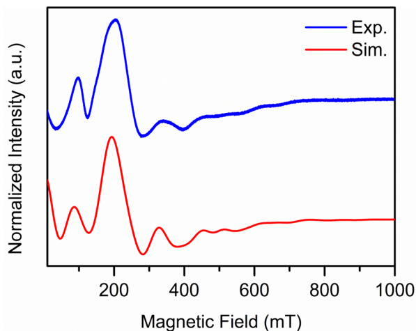
Fig. 9 Experimental (blue) and simulated (red) cw-EPR spectrum of \{[\text{Cp}_2^*\text{Ln}(\text{bpy})][\text{BPh}_4]\}_n , 1 , at 110 K collected on finely ground crystalline solids. The experimental spectrum was simulated using the parameters: S = 7/2 , g = 2.0871 , D = 0.09186 \text{ cm}^{-1} , E = 0.02269 \text{ cm}^{-1} and lwpp = 48 .
