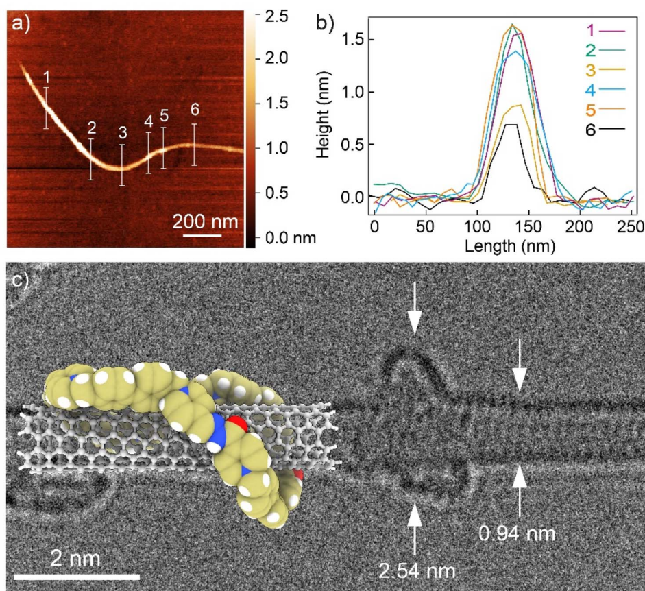
Fig. 5 (a) AFM topographic image of an eW-SWNT suspension in iPrOH and (b) height profiles along the lines marked in (a). (c) AC-HRTEM image of a SWNT containing a macrocycle (acceleration voltage 60 kV) and [2 + 2] eW-SWNT optimized structure.
