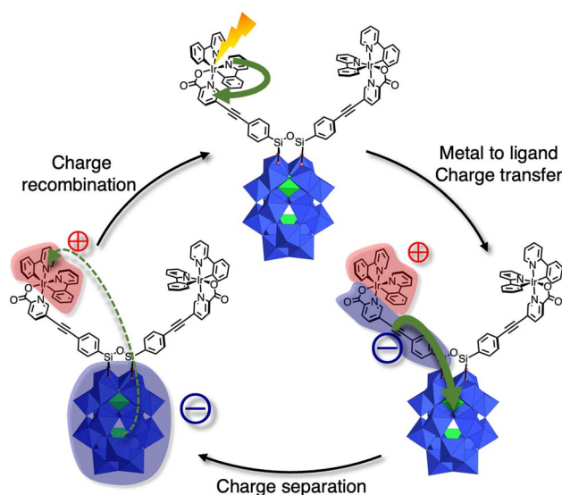
Fig. 5 Directionality in the photoinduced electron transfers of the POM-Ir(III) assembly [P_2W_{17}O_{61}\{O(SiC_3H_2O_2N_3Ir)_2\}]^{6-} , conferred by the heteroleptic character of the Ir(III) complex. The red and blue cloud respectively represent the localization of the positive and negative charges in the different excited states. 51
