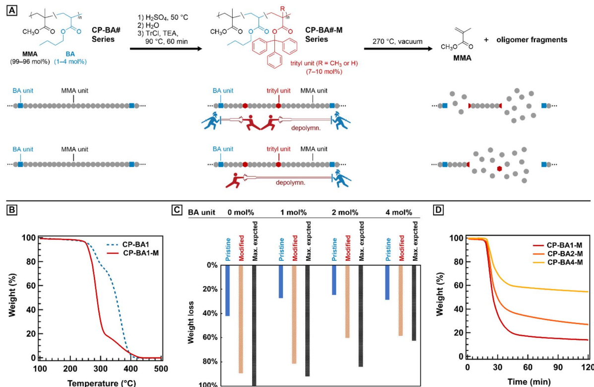
Fig. 6 (A) Pendant modification of poly(MMA-co-BA) and the monomer recovery via depolymerization. (B) TG curves of CP-BA1 and CP-BA1-M (heating ratio of 10\text{ }^\circ\text{C min}^{-1} ). (C) Weight losses of pristine and modified (co)polymers at 320\text{ }^\circ\text{C} in TG curves and their maximum expected values. (D) TG curves of CP-BA1-M–CP-BA4-M under constant temperature conditions of 270\text{ }^\circ\text{C} .
